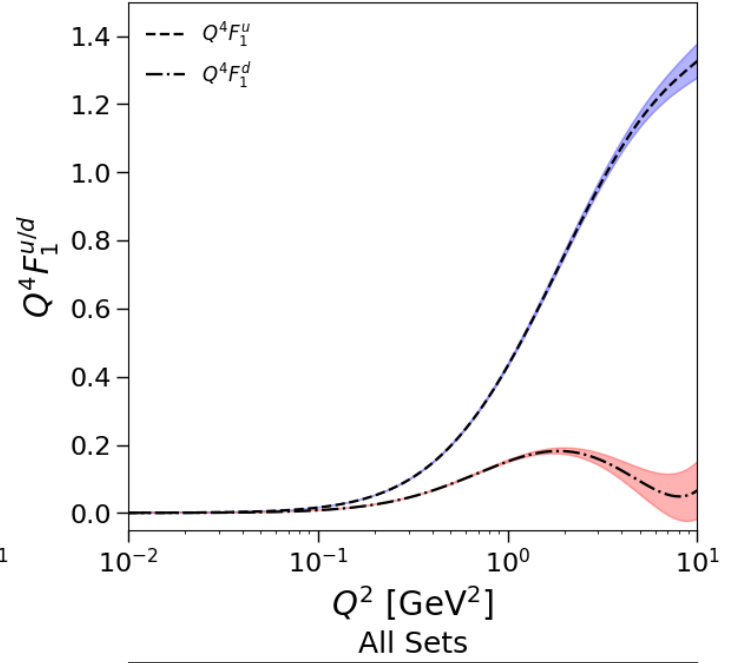
Updated with SBS G_M^n
